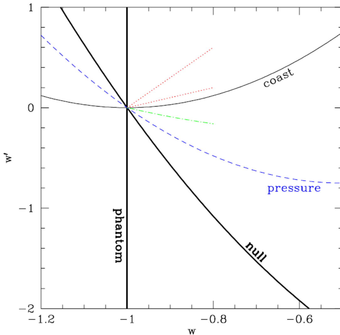
Figure 1: The dynamical phase space w-w' is divided by three curves defined by physical conditions: the phantom line w = -1 , the null line w' = -3(1-w^2) following from a flat potential, and the coasting line w' = 3(1+w)^2 following from constant field velocity. These extend across the phase space.
