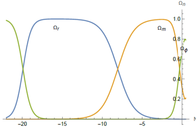
Figure 4: Evolution of the \Omega_n for Hilltop Quintessence
